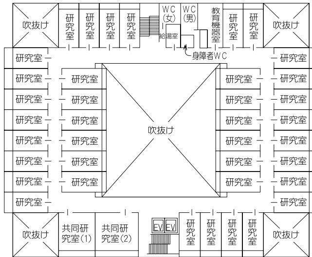
4階 (1,396㎡)
