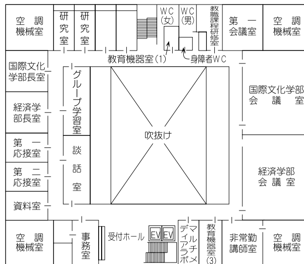
3 階 (1,319m 2 )
