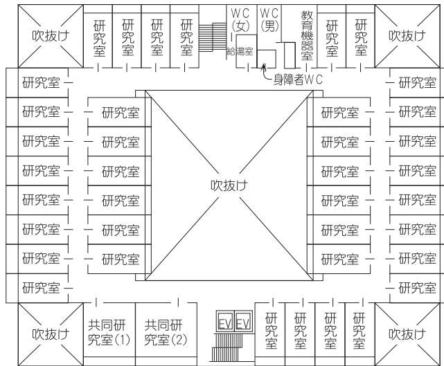
4 階 (1,396m 2 )
