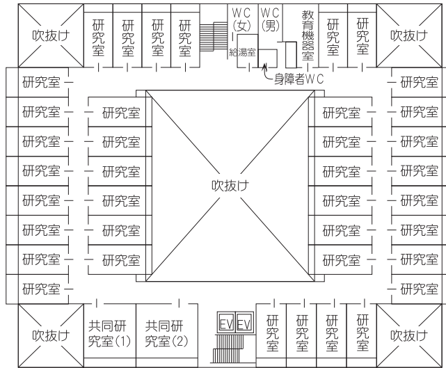
5 階 (1,396m 2 )
